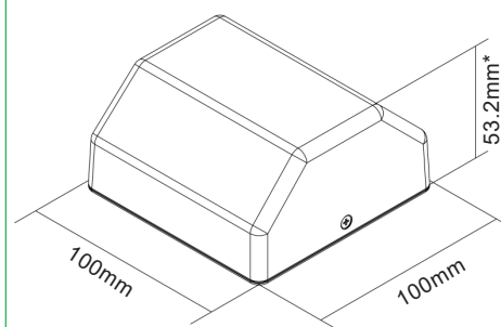
External dimensions
